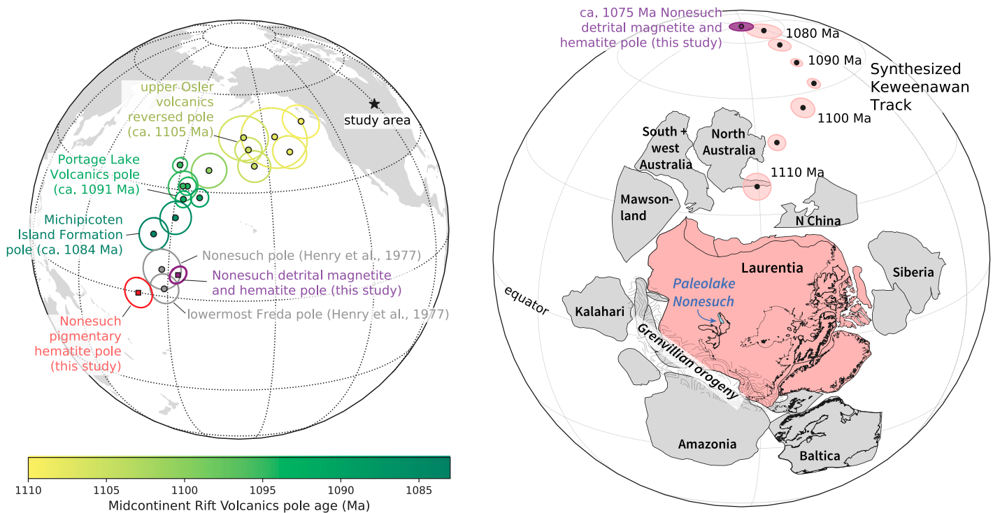
Figure 7. Left panel: Paleomagnetic poles from this work compared with those from the literature for the Midcontinent Rift (pole compilation from Swanson-Hysell, 2021). Note that our inclination-corrected Nonesuch detrital pole location agrees within uncertainty with that of Henry et al. (1977). The new detrital magnetization pole has an uncertainty that is smaller due to the increased number of samples and is elliptical in shape due to the incorporation of flattening factor uncertainty using the method of Pierce et al. (2022). The pigmentary hematite pole is in a distinct position and formed following deposition during burial after plate motion slowed due to the Grenvillian orogeny. Right panel: Paleogeography of Laurentia and associated continents during deposition of the Nonesuch Formation (modified from Swanson-Hysell et al., 2023). Paleolake Nonesuch is shown as a minimum extent that encircles the outcrop exposures of the Nonesuch Formation in northern Wisconsin and Michigan. The lake was at a tropical latitude in the interior of Laurentia (cratonic North America), which was conjoined with other continents in the supercontinent Rodinia.
