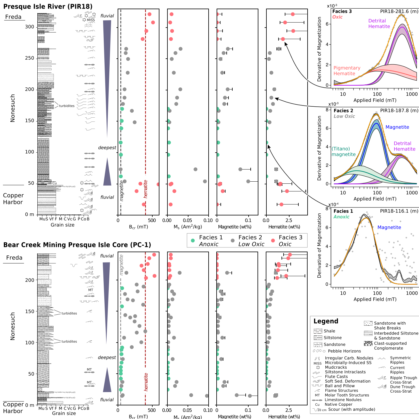
Figure 3. Stratigraphic sections with sedimentological observations, magnetic data, and facies interpretations from Presque Isle River and nearby drill core PC-1 are shown. These data constrain an abrupt deepening into the lake before progressive shallowing into marginal lacustrine facies and, eventually, into fluvial sediments as shown schematically with blue triangles. Magnetic parameters and the quantification of magnetic minerals (see Appendix for methodology) delineate three magnetic facies linked to environmental conditions. Example representative coercivity spectra are shown for each of the three magnetic facies. Note the change in y-axis scale for the Facies 1 example due to an order-of-magnitude weaker magnetization. B_{cr} —coercivity of remanence; M_s —saturation magnetization; Mu—mudstone; S—siltstone; Vf—very-fine-grained sandstone; F—fine-grained sandstone; M—medium-grained sandstone; C—coarse-grained sandstone; Vc—very-coarse-grained sandstone; G—granule conglomerate; P—pebble conglomerate; Co—cobble conglomerate; B—boulder conglomerate; Carb.—carbonate; SS—sedimentary structure; Sed.—sediment; Cross-Strat—cross-stratification.
