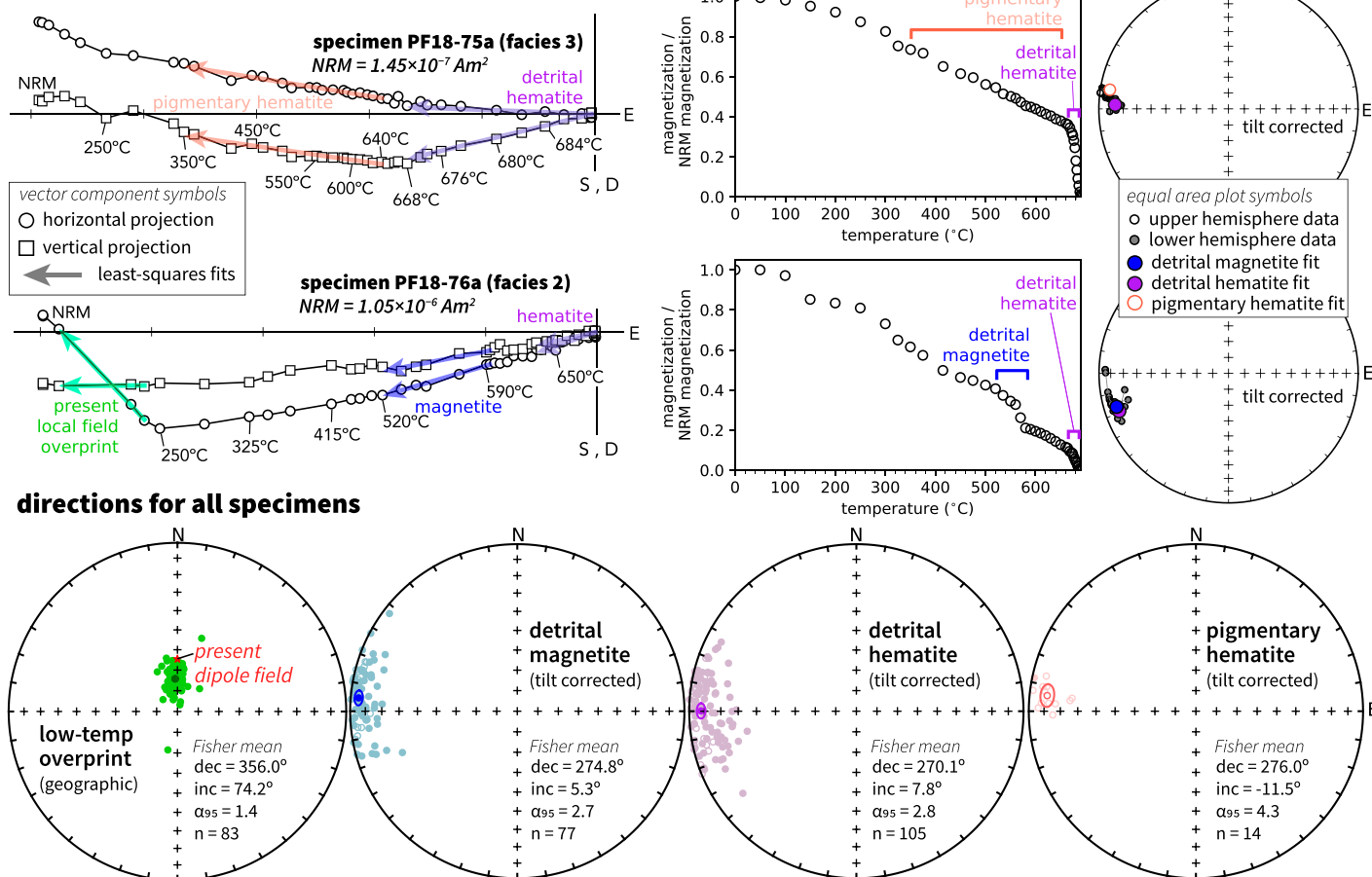
Figure 6. Thermal demagnetization paleomagnetic data for a specimen from Facies 3 (PF18-75a) and a specimen from Facies 2 (PF18-76a) are shown as vector component plots, magnetic moment plots, and equal area plots. The Facies 3 data have a well-resolved high unblocking temperature component (consistent with being held by detrital hematite) and a component that progressively unblocks up to \sim 660^\circ\text{C} (consistent with being held by pigmentary hematite) that is in a distinct direction. The Facies 2 data reveal components held by magnetite and high unblocking temperature hematite that give similar directions—consistent with a primary detrital remanent magnetization held by two different magnetic minerals. Directions for siltstone to very fine sandstone specimens analyzed and fit with the different components are shown in the equal area plots in the bottom panel. The low-temperature overprint has a similar direction to that of the present local field. The detrital magnetite and detrital hematite directions are both west and shallowly down. The pigmentary hematite direction is similar to but distinct from the detrital remanence direction. NRM—natural remanent magnetization; temp—temperature; dec—declination; inc—inclination; n—number of directions used in the mean.
