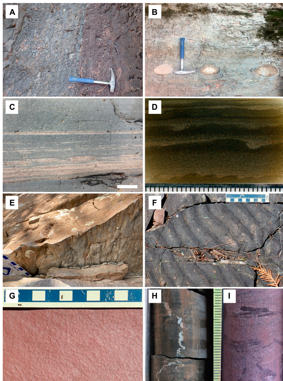
Figure 5. (A) Color change from magnetic Facies 3 with pigmentary hematite on the right into magnetic Facies 2 on the left. The beds are steeply dipping with stratigraphic up-direction to the left (82.0 m in section DG18; hammer is 33 cm long). (B) Limestone nodules within siltstone of the Nonesuch Formation correspond to magnetic Facies 1 (~94 m in section PIR18). Differential compaction of the siltstone bedding around the nodules indicates that they formed early within the sediment. (C) Sediment-starved current ripples (tan colored) of very fine to fine sand within gray siltstone (between 70 m and 100 m in section PRF18; white bar is 2 cm). (D) Fining-upward packages and dewatering structures give the siltstone to very fine sandstone a wavy lamination, as seen in a thin section scan (78.1 m in section PRF18; ticks are 1 mm). (E) Flute casts at the base of a turbidite (~170 m in section PIR18, scale bar is in cm). (F) Oscillatory wave ripples in the uppermost Nonesuch Formation (298.5 m in section PIR18; scale bar rectangles are 1 cm). (G) Crinkly texture on siltstone/very fine sandstone that could be the result of a microbial mat and therefore a microbially induced sedimentary structure (307.7 m in section PIR18; scale bar rectangles are 1 cm). (H) Molar tooth structure in PC-1 core (depth of 306 ft; ticks are 1 mm). (I) Cross-stratified fluvial sandstone in PC-1 core with red siltstone rip-up clasts (depth of 133 ft; same scale as in panel H, with 1 mm ticks).
