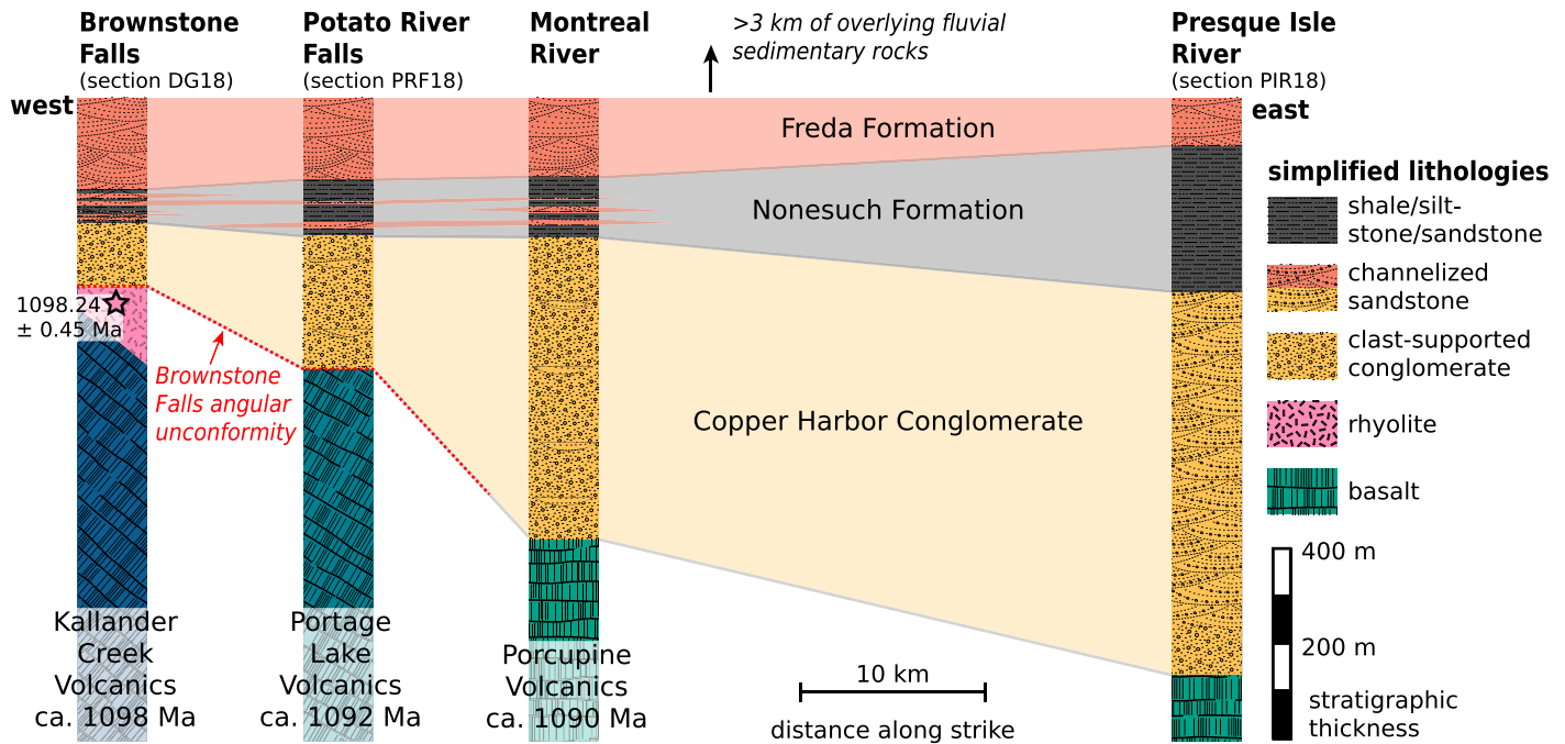
Figure 2. Summary of lithostratigraphy across the outcrop study region illustrates the change in formation thicknesses. The corresponding stratigraphic sections through the Nonesuch Formation shown in Figures 3 and 4 are written above each column. Where the Nonesuch Formation is thickest and consists of a single deepening- and shallowing-upward succession (at the Presque Isle River; section PIR18), the underlying Copper Harbor Conglomerate is also at its thickest. Both formations thin toward the paleotopographic high at Brownstone Falls, where the DG18 section was measured (Fig. 1). Close to the paleotopographic high, the Nonesuch Formation records multiple transitions into and out of fluvial and lacustrine environments. These section locations near the paleotopographic high would have repeatedly been the shoreline, while there was a continuously subaqueous environment to the east at the Presque Isle River section.
