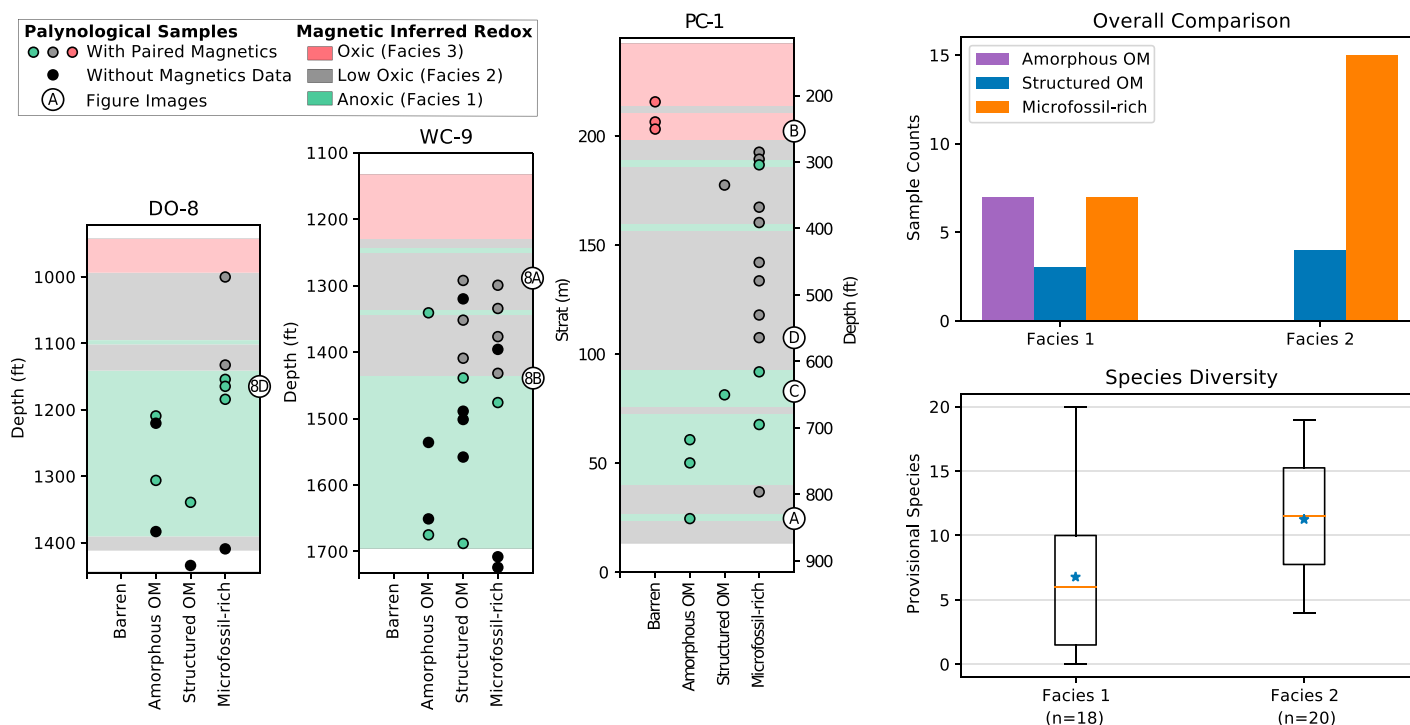
Figure 10. Palynological data of three drill cores are shown in the context of stratigraphic position and magnetic mineralogy-based redox interpretations. Organic matter (OM) was categorized into one of four categories: barren; amorphous (sometimes in chunks suggestive of microbial mats), with no (or in one case rare) microfossils; structured, with low-density scrappy palynomorphs that can be difficult to identify; and microfossil-rich. Stratigraphic plots show these categorized samples, which are color-coded by redox if paired magnetic measurements were made; broad redox interpretations are indicated by the background colors. Microfossil images from DO-8 and WC-9 in Figure 8 and organic matter classification images from PC-1 in Figure S12 (see text footnote 1) are keyed via text in circles on the right side of the plots. The histogram in the upper right highlights that anoxic Facies 1 contains more amorphous organic matter than low-oxic Facies 2, which has more microfossil-rich samples. Species diversity is typically greater in Facies 2, as seen in the box plot in the lower right. The box represents the lower and upper quartiles of the number of provisional species, with the orange line indicating the median, the blue star indicating the mean, and whiskers showing the range of the data.
