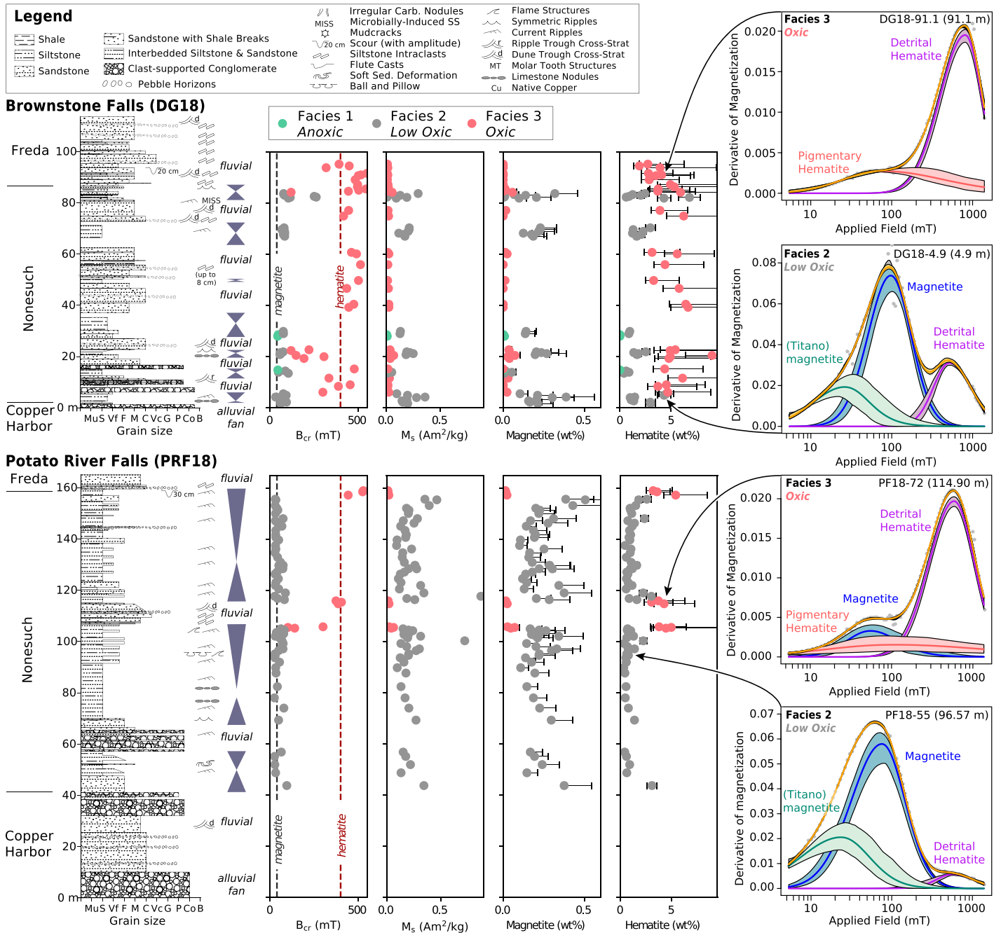
Figure 4. Stratigraphic observations, magnetic data, and facies interpretations from the Brownstone Falls (DG18) and Potato River Falls (PRF18) outcrop sections are shown. These sections reveal several packages of lacustrine deposition separated by fluvial sediments. The interpretation of deepening and shallowing into and out of fluvial and lacustrine systems is shown with blue triangles. Magnetic parameters and the absolute quantification of magnetic minerals allowed for separation of samples into three magnetic facies linked to environmental conditions. Example representative coercivity spectra are shown for each magnetic facies within each section. Note that the scales for M_s , magnetite (wt%), and hematite (wt%) are distinct from those in Figure 3. The two samples with the highest M_s values in PRF18 are off-scale in the magnetite (wt%) plot. See Figure 3 for abbreviations.
