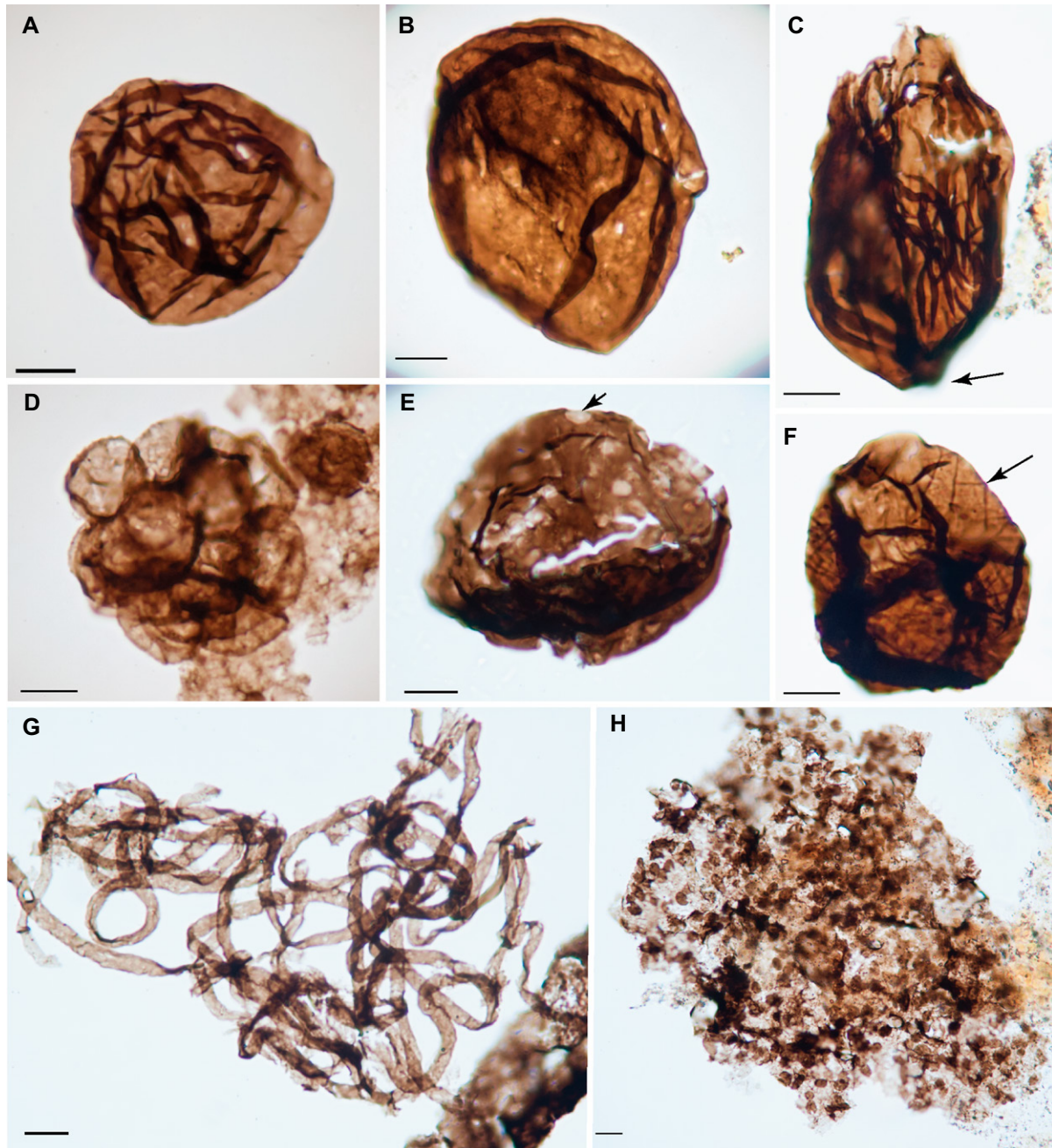
Figure 8. Images show examples of palynomorphs from the Nonesuch Formation mentioned in the text (all scale bars are 10 \mu\text{m} ). (A) Leiosphaeridia crassa from WC-9, 1292 ft (sample NON18-79), is a common sphaeromorph acritarch in the assemblage. Note the compression folds likely associated with flattening of an original spherical shape. (B) Valeria lophostriata from WC-9, 1439 ft (sample NON18-64), is a sphaeromorph characterized by its wall pattern of fine concentric laminae, just barely visible here (see Strother and Wellman, 2021, for a close-up of striations in another specimen from the Nonesuch Formation). (C) Unnamed elongate protist from the Big Iron River outcrop section (sample NON18-89) with a basal attachment scar (indicated with arrow) suggesting the presence of a stalk. This morphology suggests that the protist was a benthic organism. (D) (Multi)cellular cluster, similar in morphology to the reproductive stages of living basal Holozoa, from DO-8, 1164.5 ft (sample NON18-14). (E) Holes (one of which is indicated with arrow) in a microfossil from the Big Iron River outcrop section (sample NON18-114). These perforations could be the result of predation, possibly from chytrids. (F) Possible euglenid characterized by helical striae that wrap around the wall (arrow) from the Big Iron River outcrop section (sample NON18-115). (G) Mass of entangled Siphonophycus , a cyanobacterial sheath, that was likely derived from a microbial mat rip-up from the Big Iron River outcrop section (NON18-114). (H) Cells of the planktonic cyanobacterium Eohalotheca lacustrina from the Big Iron River outcrop section (sample NON18-111) embedded in organic material, which is potentially a remnant of a microbial mat.
