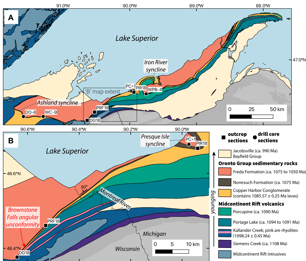
Figure 1. Geologic map shows the region where the Nonesuch Formation outcrops and was studied in stratigraphic drill core. (A) The full extent of the Nonesuch Formation in northern Wisconsin and the Upper Peninsula of Michigan and the locations of the studied outcrop and core sections are shown. (B) This map zooms in on the region of the Montreal River monocline from the Presque Isle River in the east to Brownstone Falls in the west, where the sedimentary rocks of the Oronto Group rest on a post-rift unconformity (Brownstone Falls angular unconformity, red line). Geologic data are from Cannon et al. (1995) and Cannon et al. (1996), with minor modifications associated with new field data. As a result of this unconformity, the Copper Harbor Conglomerate is progressively in contact with older volcanic rocks to the southwest. The Copper Harbor Conglomerate and the Nonesuch Formation progressively thin to the southwest against this uncon-
